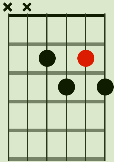
1st inversion
