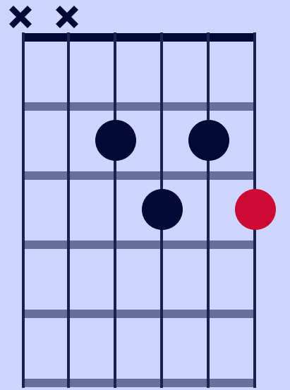
3rd inversion
